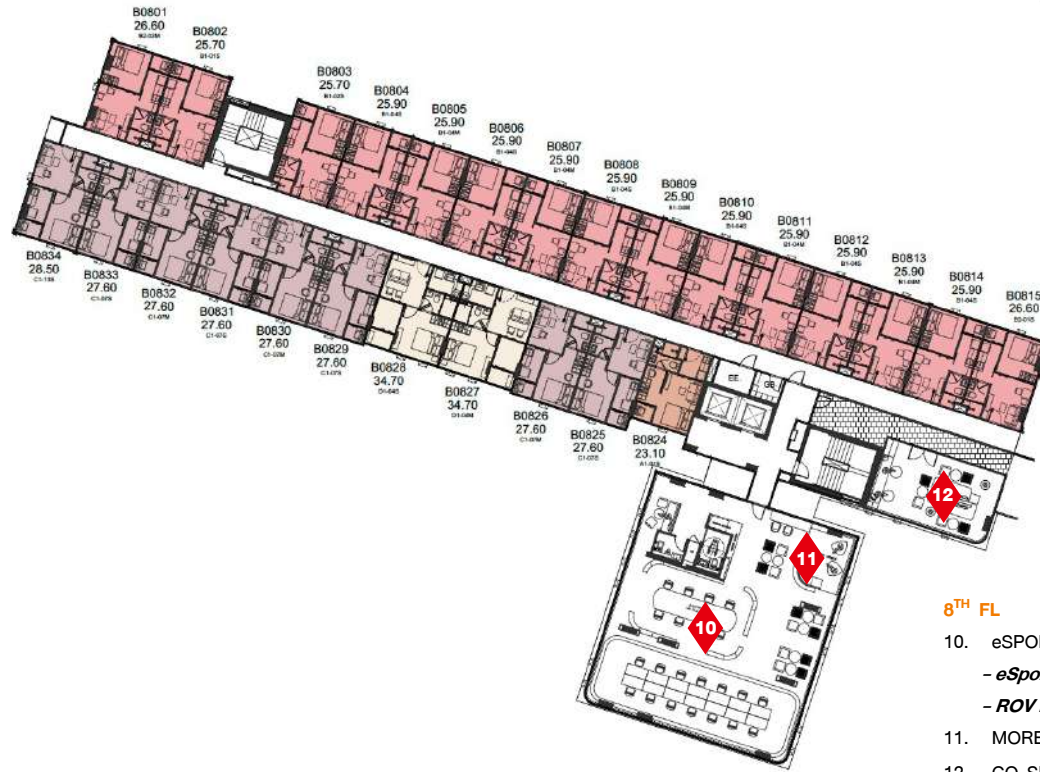
8 th Floor
