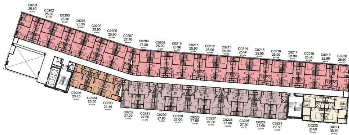
2 nd Floor
